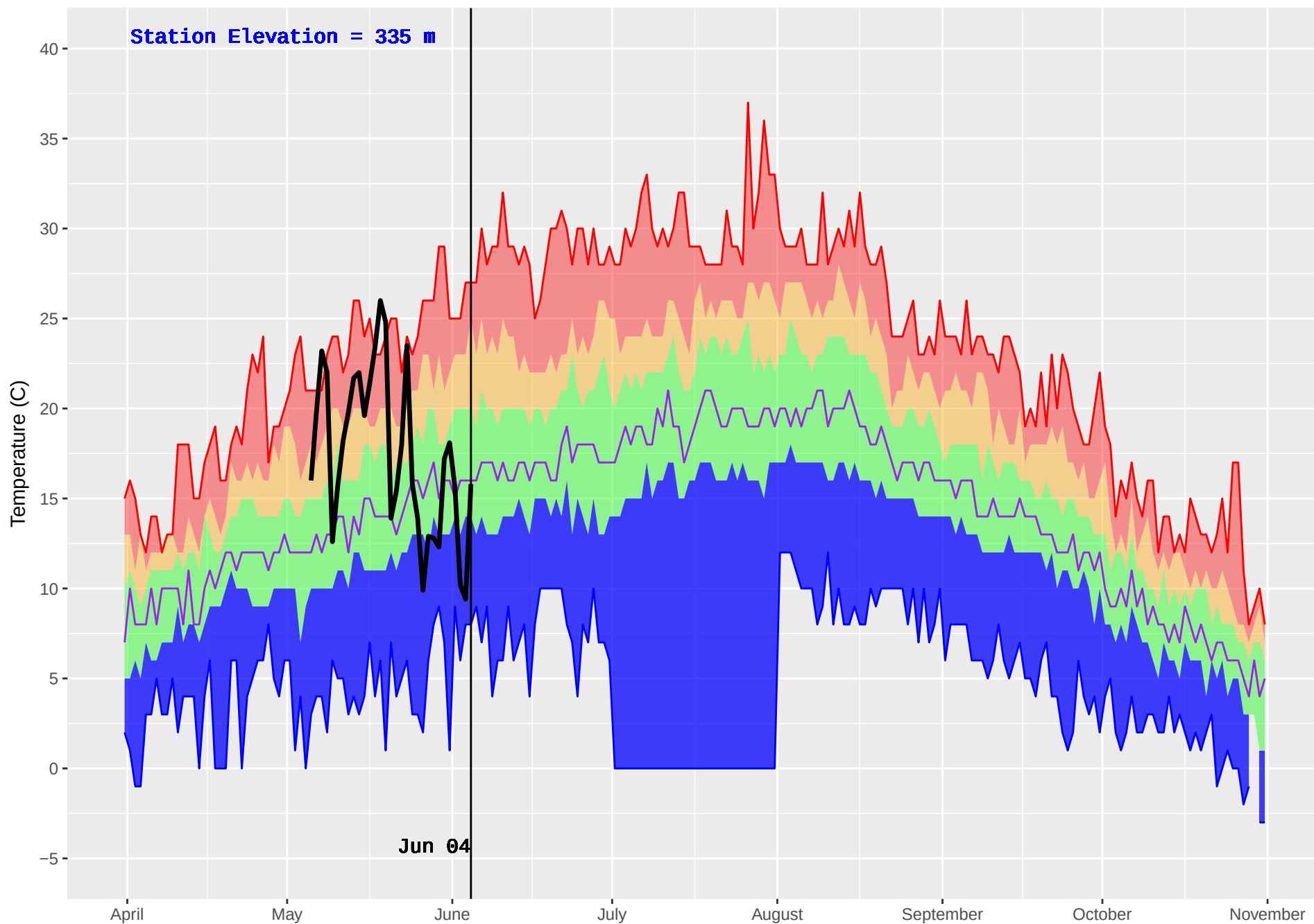
KISPIOX HUB (428) : Historical (1970–2016) and Current (2018) Noon Temperature
