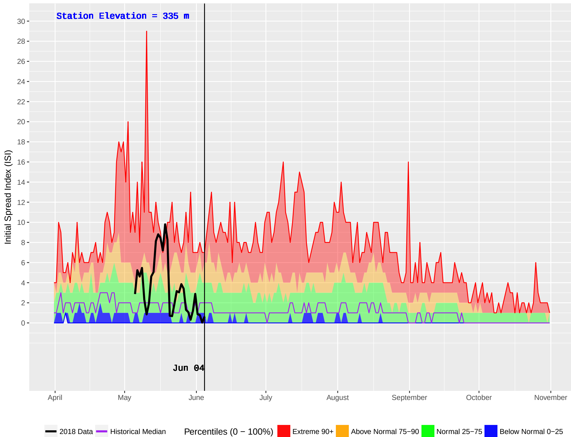
KISPIOX HUB (428) : Historical (1970–2016) and Current (2018) Noon Initial Spread Index (ISI)
