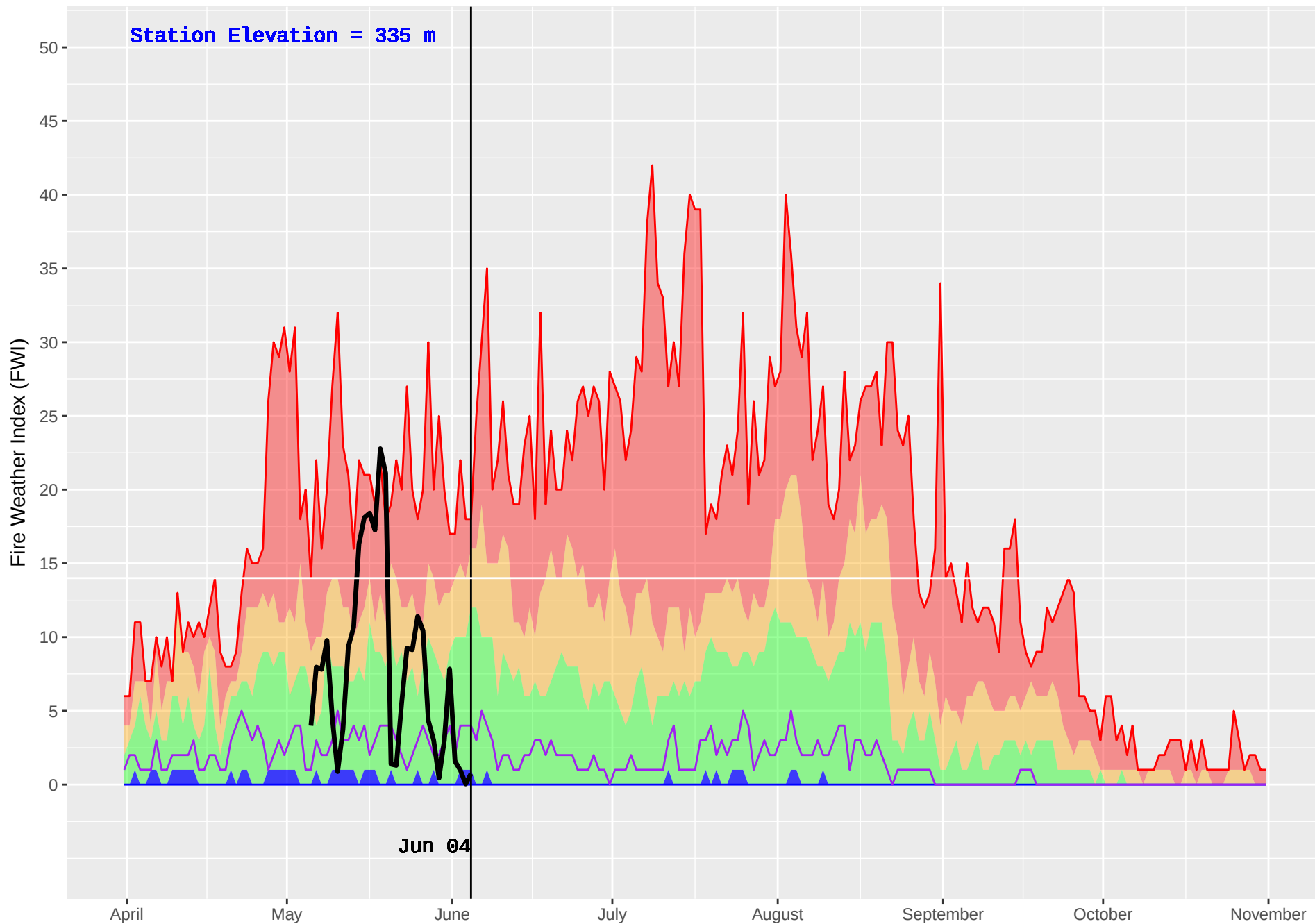
KISPIOX HUB (428) : Historical (1970–2016) and Current (2018) Noon Fire Weather Index (FWI)
