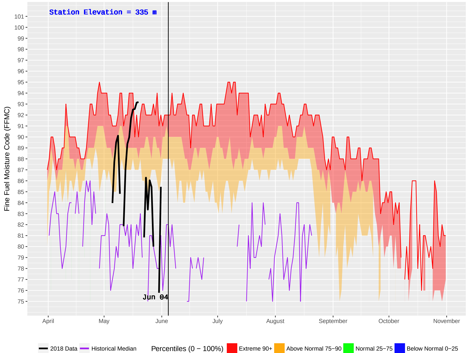
KISPIOX HUB (428) : Historical (1970–2016) and Current (2018) Noon Fine Fuel Moisture Code (FFMC)
