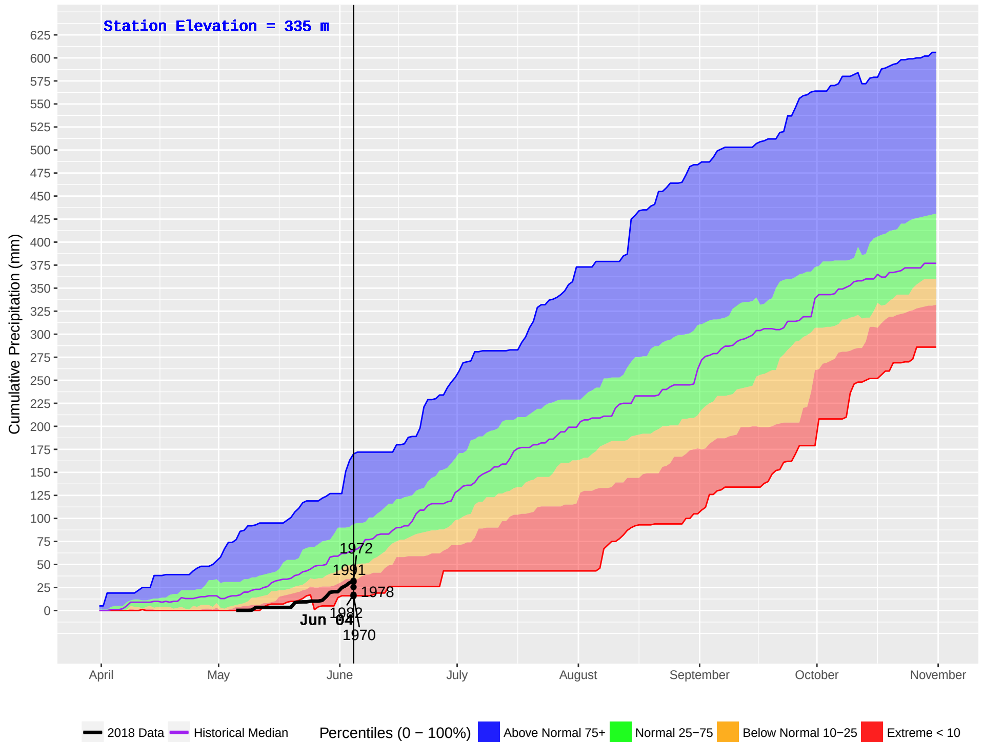
KISPIOX HUB (428) : Historical (1970–2016) and Current (2018) Noon Cumulative Precipitation
